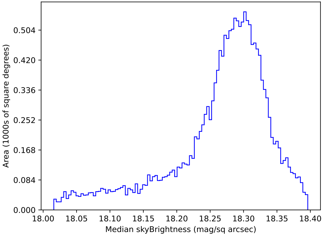
too_elab_heavy_r64_d3_ugrizy_v3.4_10yrs WFD y band: Median skyBrightness
