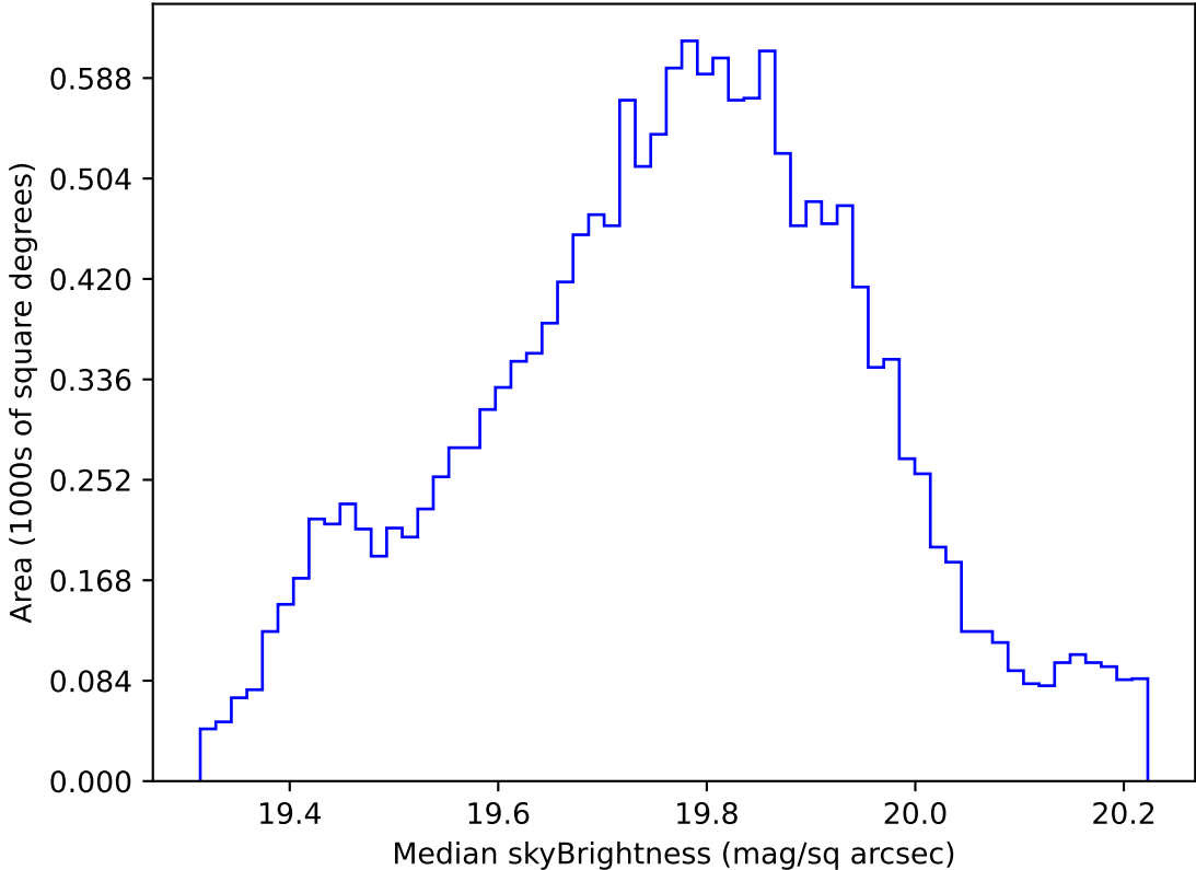
too_elab_heavy_r64_d3_ugrizy_v3.4_10yrs WFD all bands: Median skyBrightness
