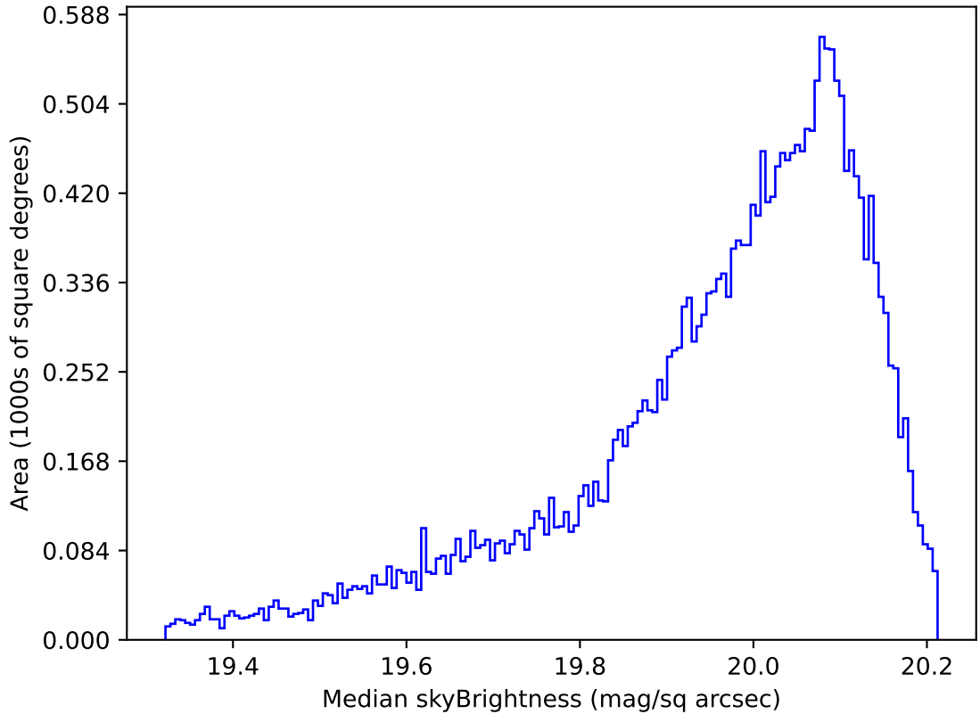
too_elab_heavy_r64_d3_ugrizy_v3.4_10yrs All sky i band: Median skyBrightness
