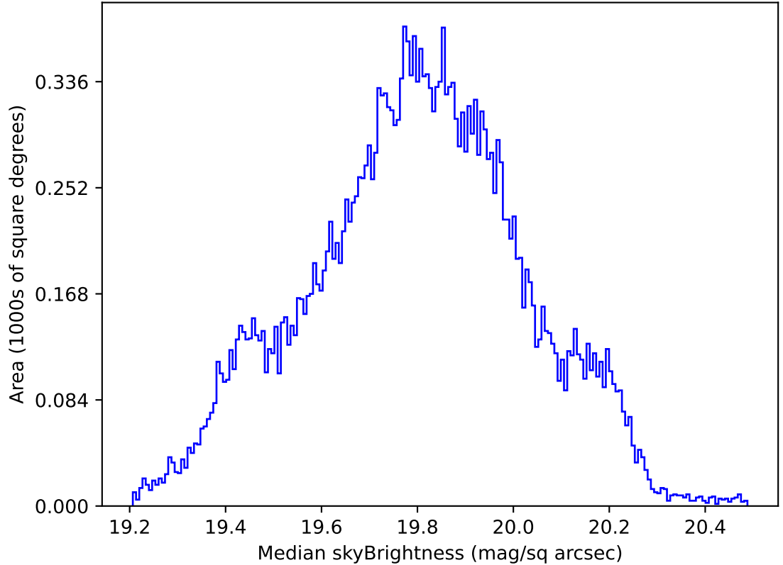
too_elab_heavy_r64_d3_ugrizy_v3.4_10yrs All sky all bands: Median skyBrightness
