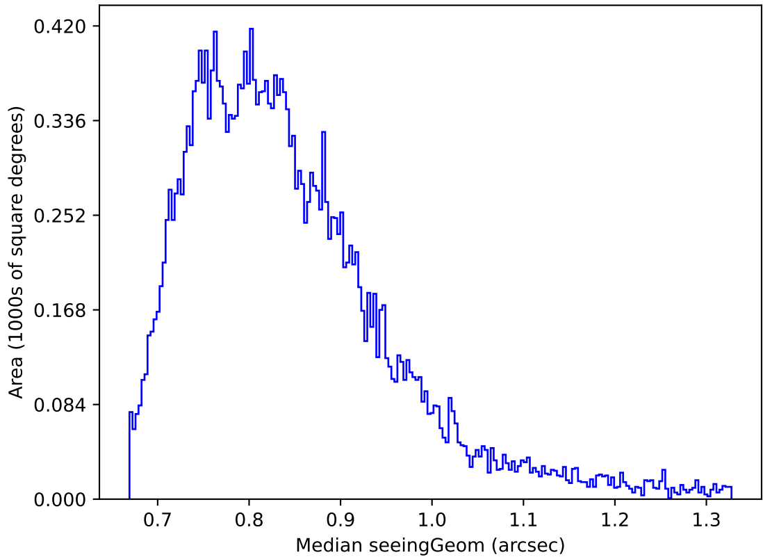
too_elab_heavy_r64_d3_ugrizy_v3.4_10yrs Yr 1 z band: Median seeingGeom
