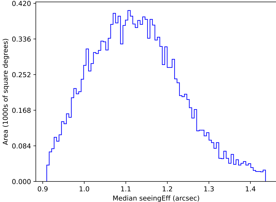
too_elab_heavy_r64_d3_ugrizy_v3.4_10yrs WFD g band: Median seeingEff
