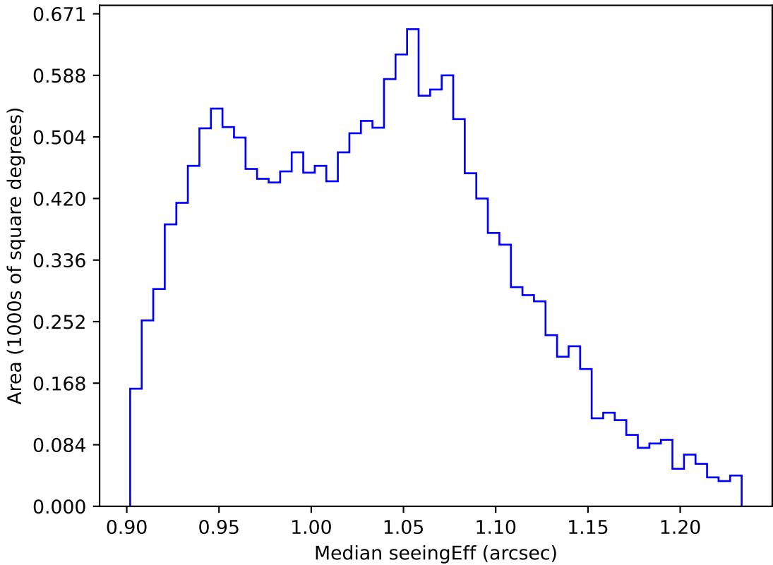
too_elab_heavy_r64_d3_ugrizy_v3.4_10yrs WFD all bands: Median seeingEff
