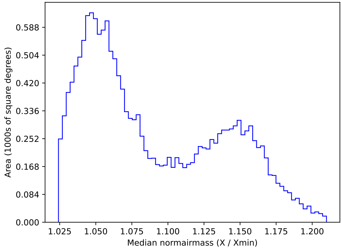
too_elab_heavy_r64_d3_ugrizy_v3.4_10yrs WFD z band: Median normairmass
