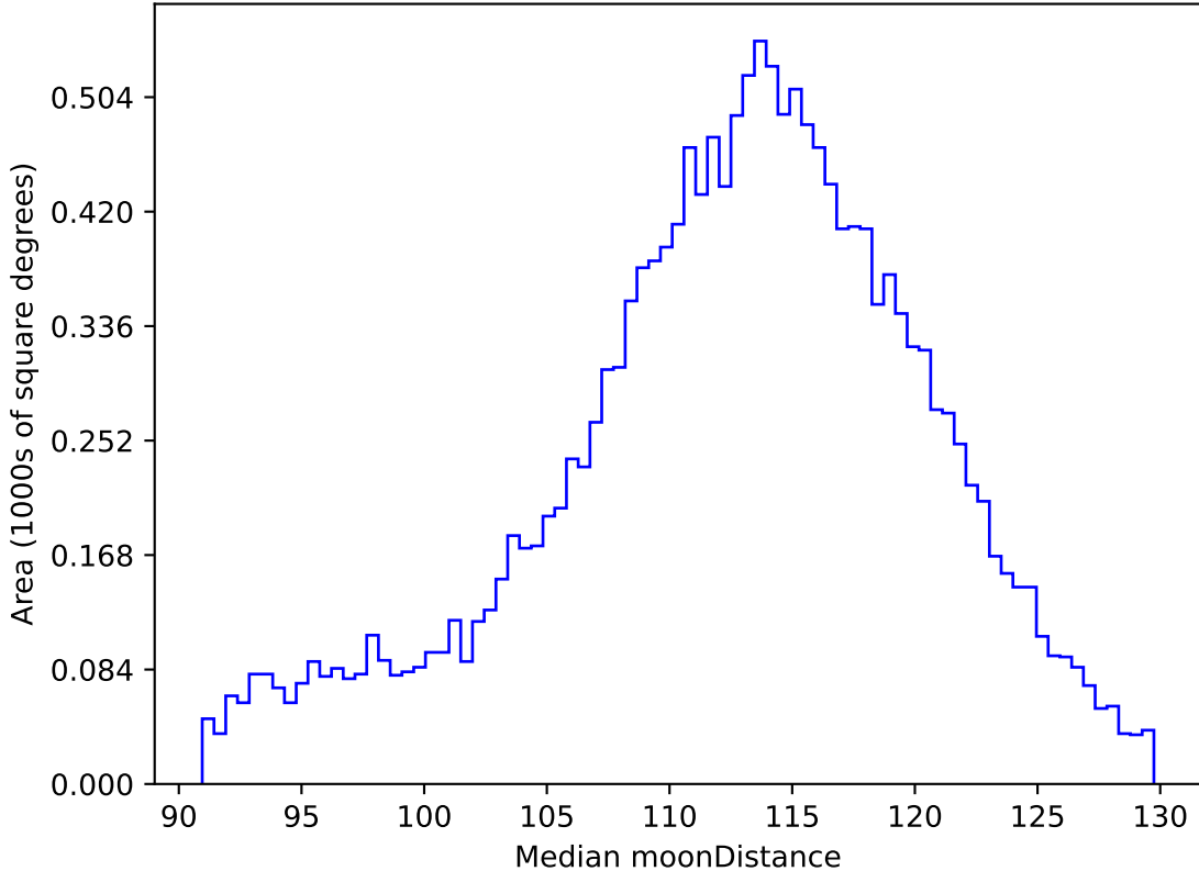
too_elab_heavy_r64_d3_ugrizy_v3.4_10yrs WFD r band: Median moonDistance
