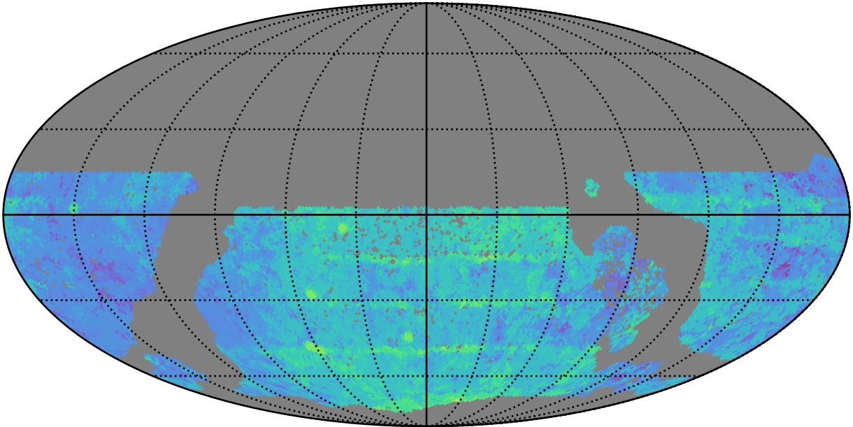
too_elab_heavy_r64_d3_ugrizy_v3.4_10yrs WFD y band: Median Season Length
