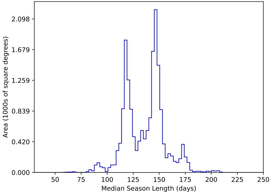
too_elab_heavy_r64_d3_ugrizy_v3.4_10yrs WFD y band: Median Season Length
