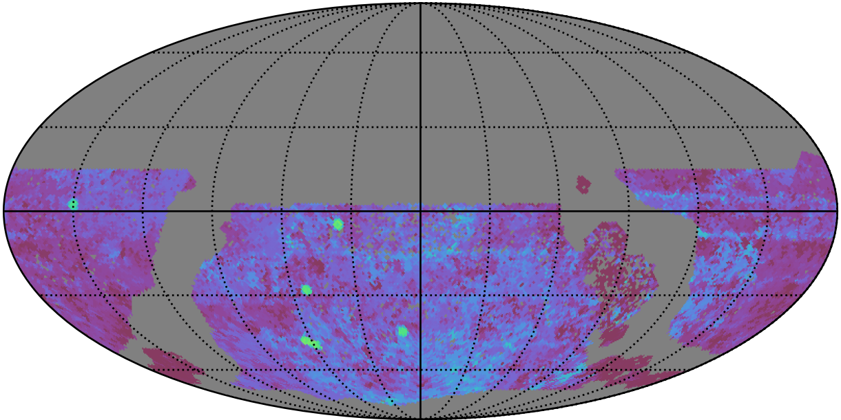
too_elab_heavy_r64_d3_ugrizy_v3.4_10yrs WFD u band: Median Season Length
