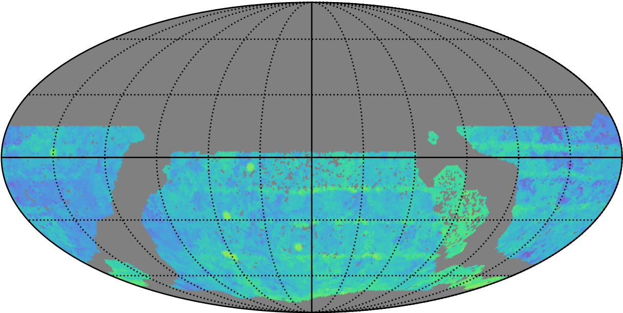
too_elab_heavy_r64_d3_ugrizy_v3.4_10yrs WFD r band: Median Season Length
