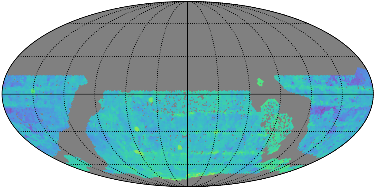
too_elab_heavy_r64_d3_ugrizy_v3.4_10yrs WFD i band: Median Season Length
