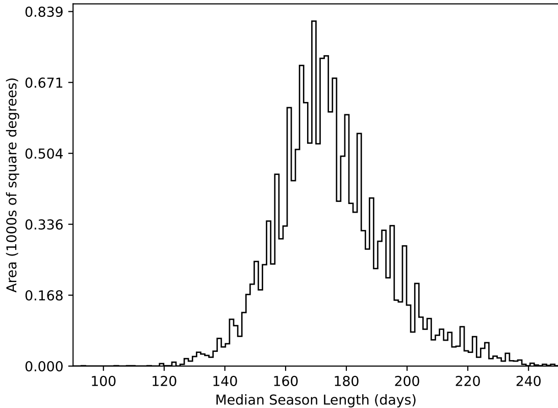
too_elab_heavy_r64_d3_ugrizy_v3.4_10yrs WFD all bands: Median Season Length
