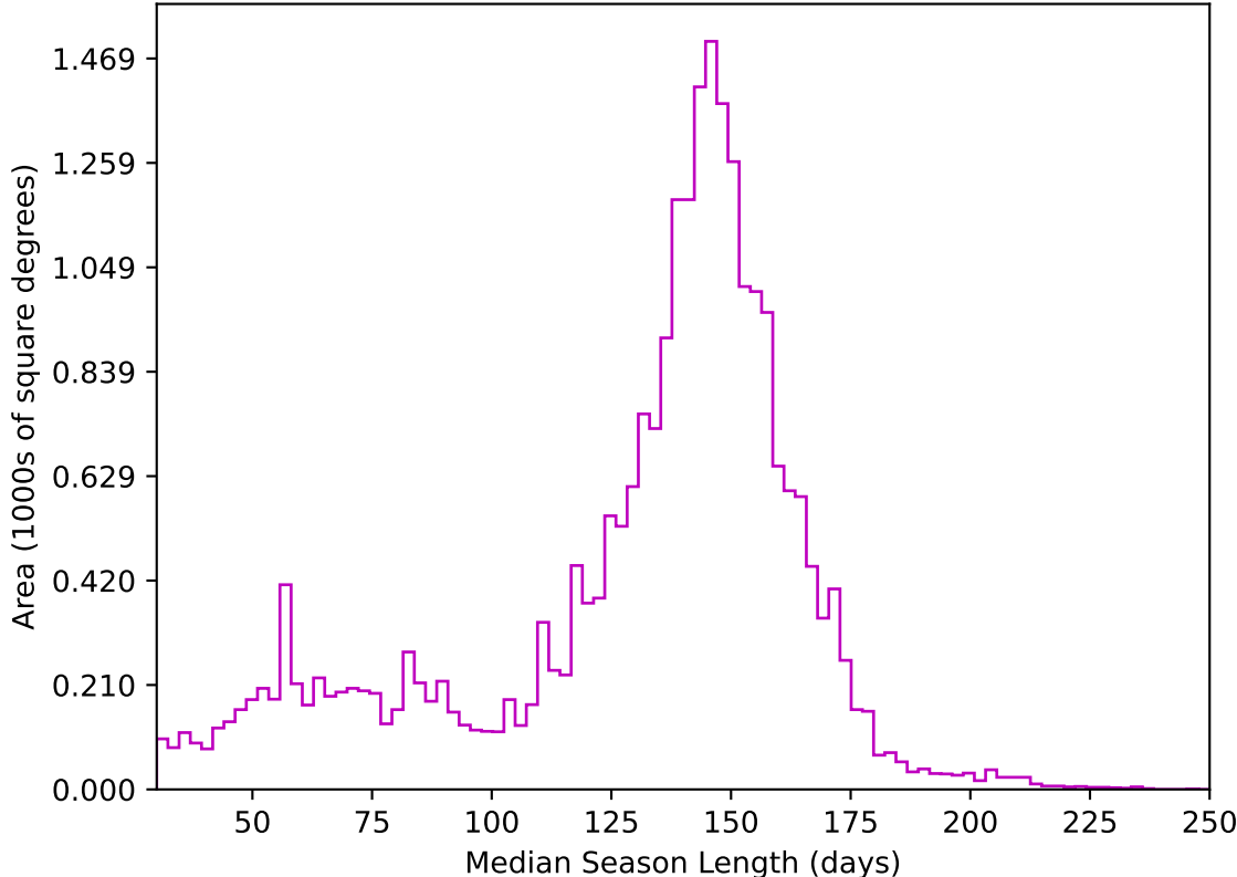
too_elab_heavy_r64_d3_ugrizy_v3.4_10yrs All sky z band: Median Season Length
