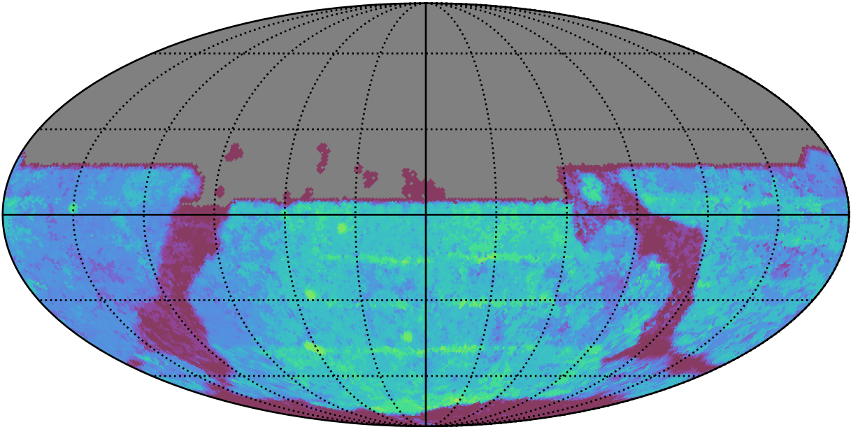
too_elab_heavy_r64_d3_ugrizy_v3.4_10yrs All sky y band: Median Season Length
