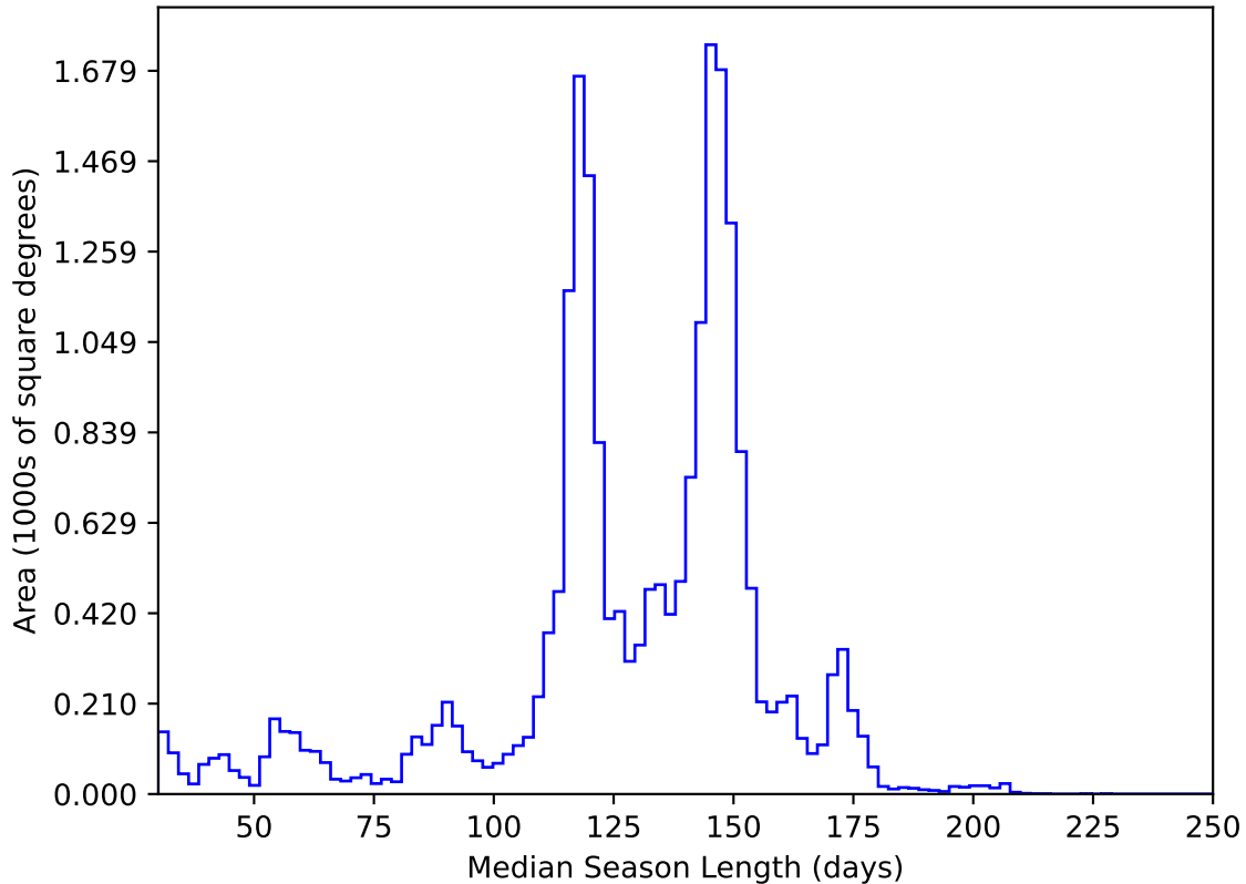
too_elab_heavy_r64_d3_ugrizy_v3.4_10yrs All sky y band: Median Season Length
