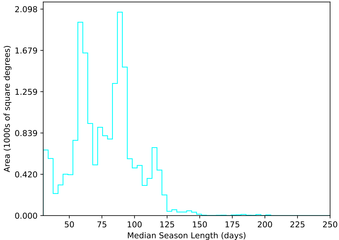
too_elab_heavy_r64_d3_ugrizy_v3.4_10yrs All sky u band: Median Season Length
