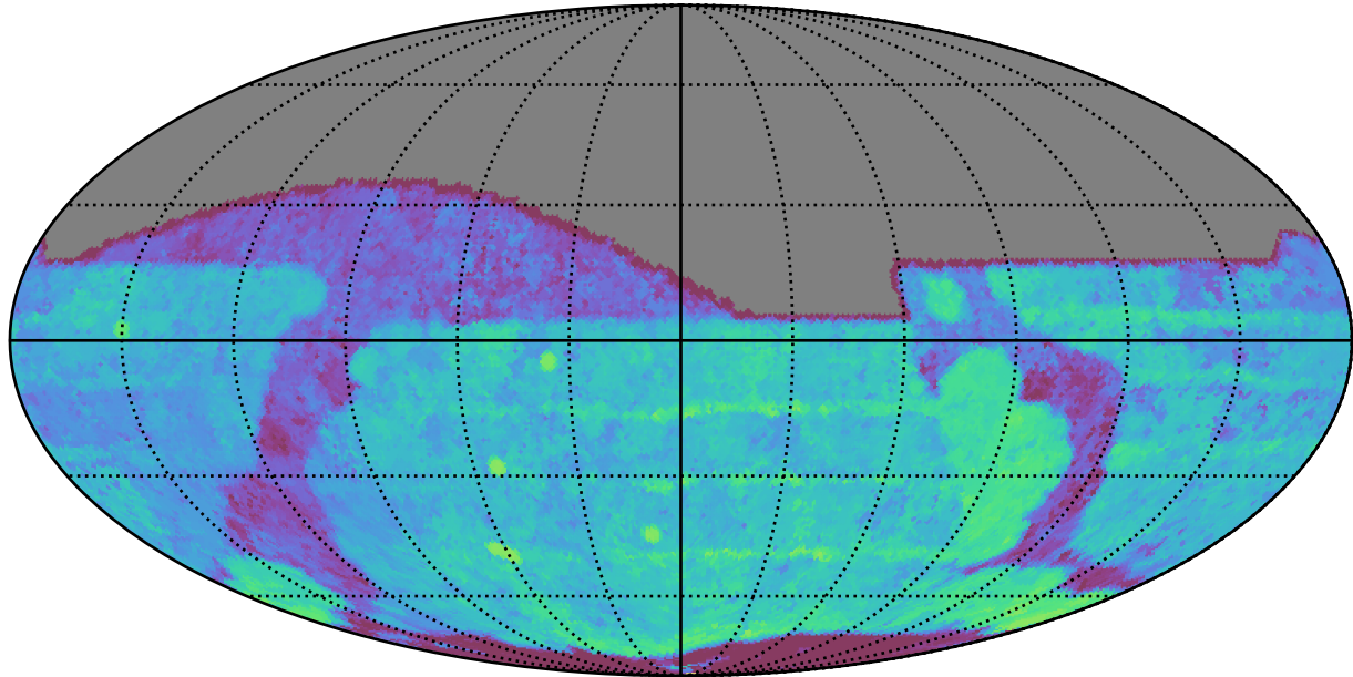
too_elab_heavy_r64_d3_ugrizy_v3.4_10yrs All sky r band: Median Season Length
