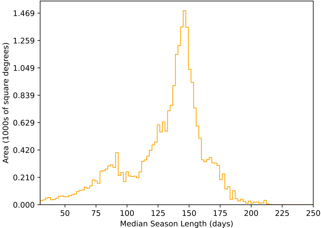
too_elab_heavy_r64_d3_ugrizy_v3.4_10yrs All sky r band: Median Season Length
