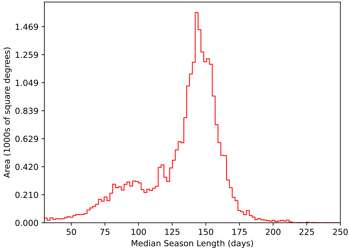
too_elab_heavy_r64_d3_ugrizy_v3.4_10yrs All sky i band: Median Season Length
