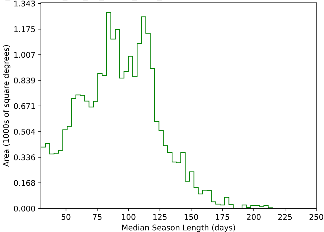
too_elab_heavy_r64_d3_ugrizy_v3.4_10yrs All sky g band: Median Season Length
