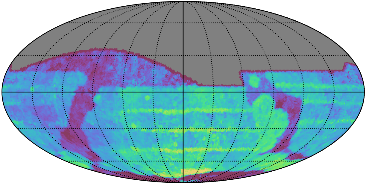
too_elab_heavy_r64_d3_ugrizy_v3.4_10yrs All sky all bands: Median Season Length
