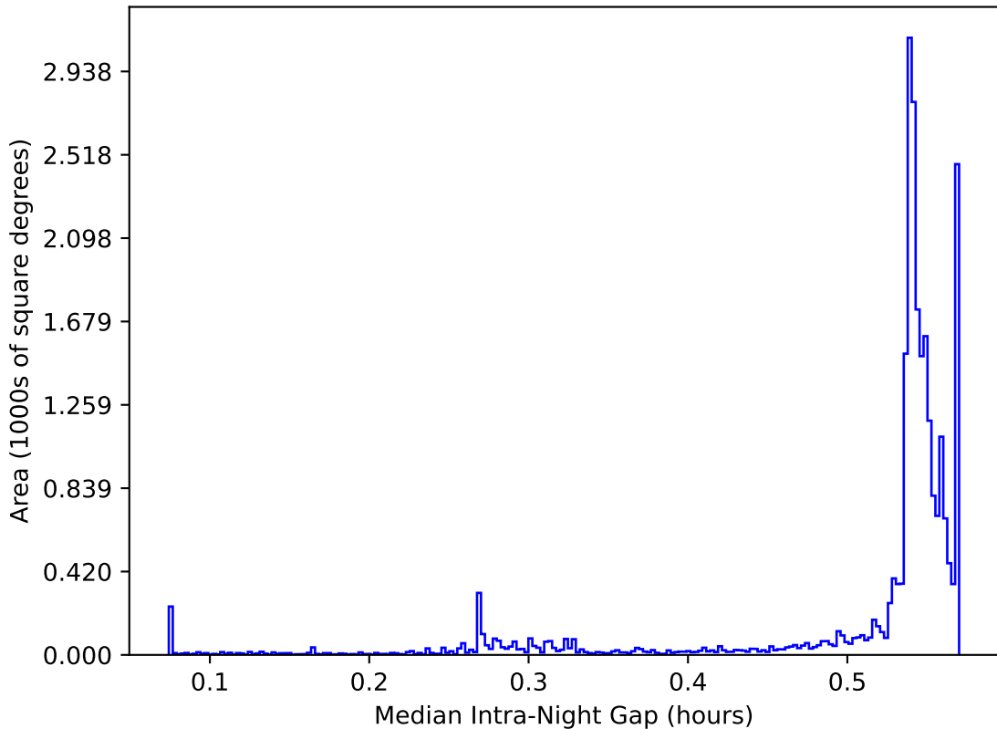
too_elab_heavy_r64_d3_ugrizy_v3.4_10yrs All sky: Median Intra-Night Gap
