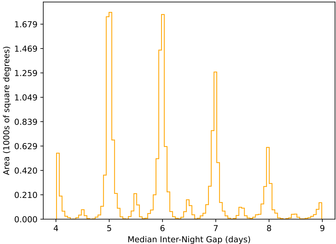
too_elab_heavy_r64_d3_ugrizy_v3.4_10yrs WFD r band: Median Inter-Night Gap
