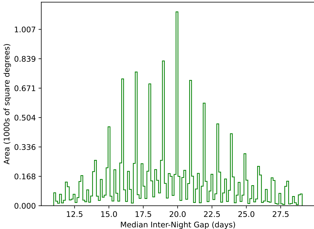
too_elab_heavy_r64_d3_ugrizy_v3.4_10yrs WFD g band: Median Inter-Night Gap
