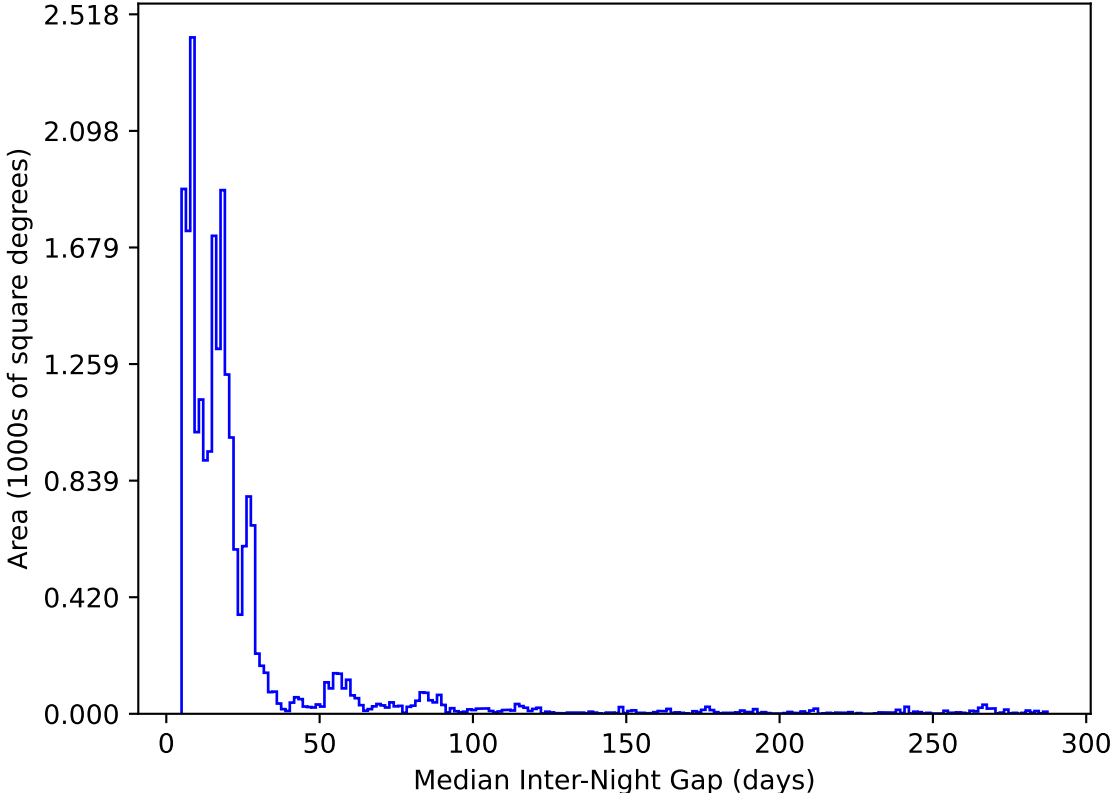
too_elab_heavy_r64_d3_ugrizy_v3.4_10yrs All sky y band: Median Inter-Night Gap
