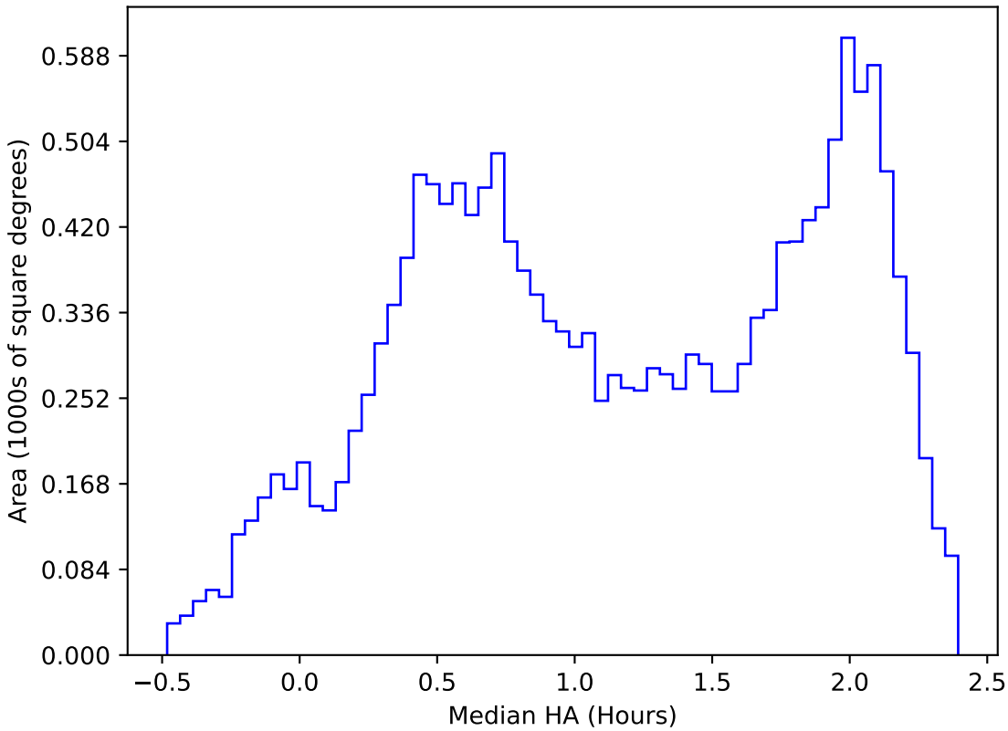
too_elab_heavy_r64_d3_ugrizy_v3.4_10yrs WFD z band: Median HA
