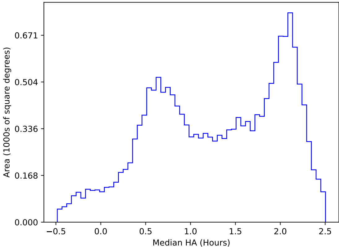
too_elab_heavy_r64_d3_ugrizy_v3.4_10yrs WFD y band: Median HA
