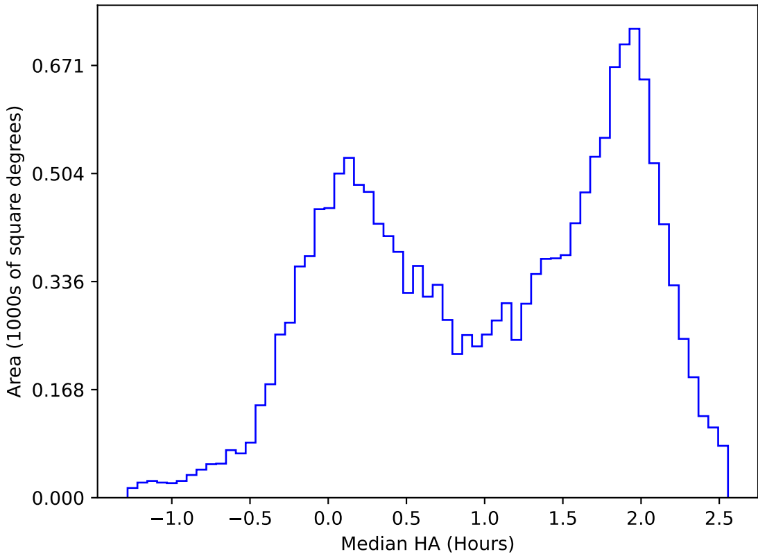
too_elab_heavy_r64_d3_ugrizy_v3.4_10yrs WFD u band: Median HA
