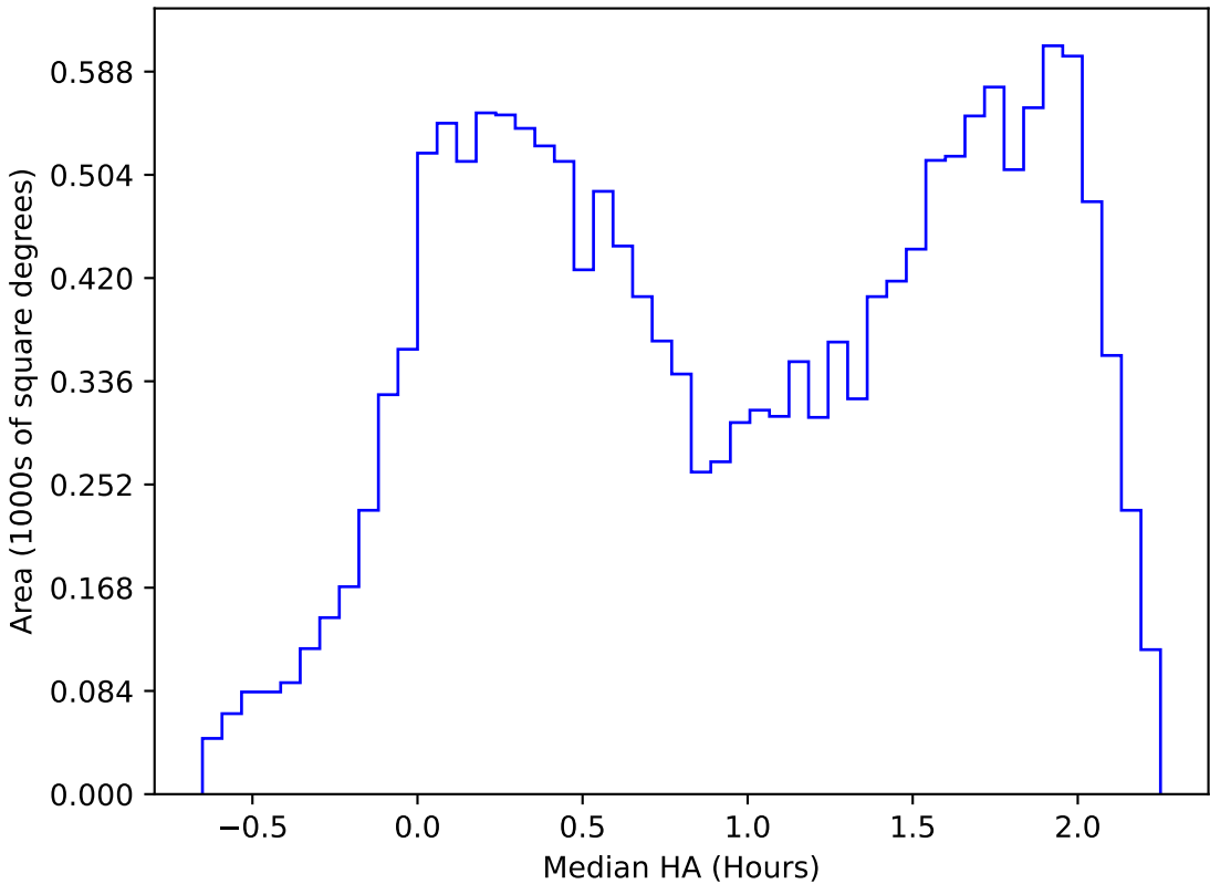
too_elab_heavy_r64_d3_ugrizy_v3.4_10yrs WFD r band: Median HA
