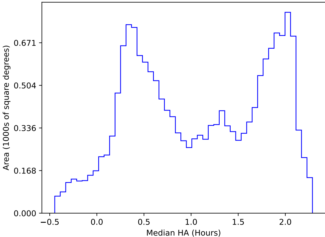
too_elab_heavy_r64_d3_ugrizy_v3.4_10yrs WFD all bands: Median HA
