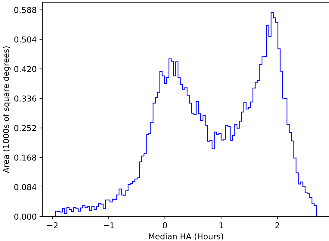
too_elab_heavy_r64_d3_ugrizy_v3.4_10yrs All sky u band: Median HA
