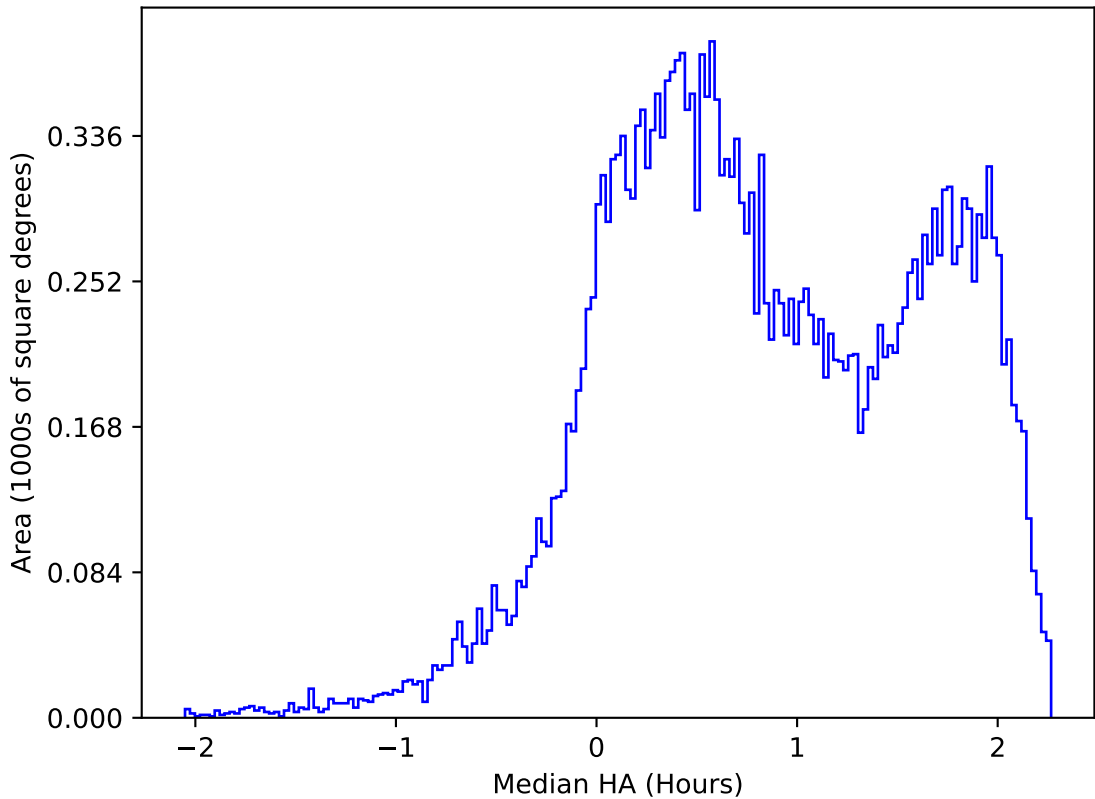
too_elab_heavy_r64_d3_ugrizy_v3.4_10yrs All sky r band: Median HA
