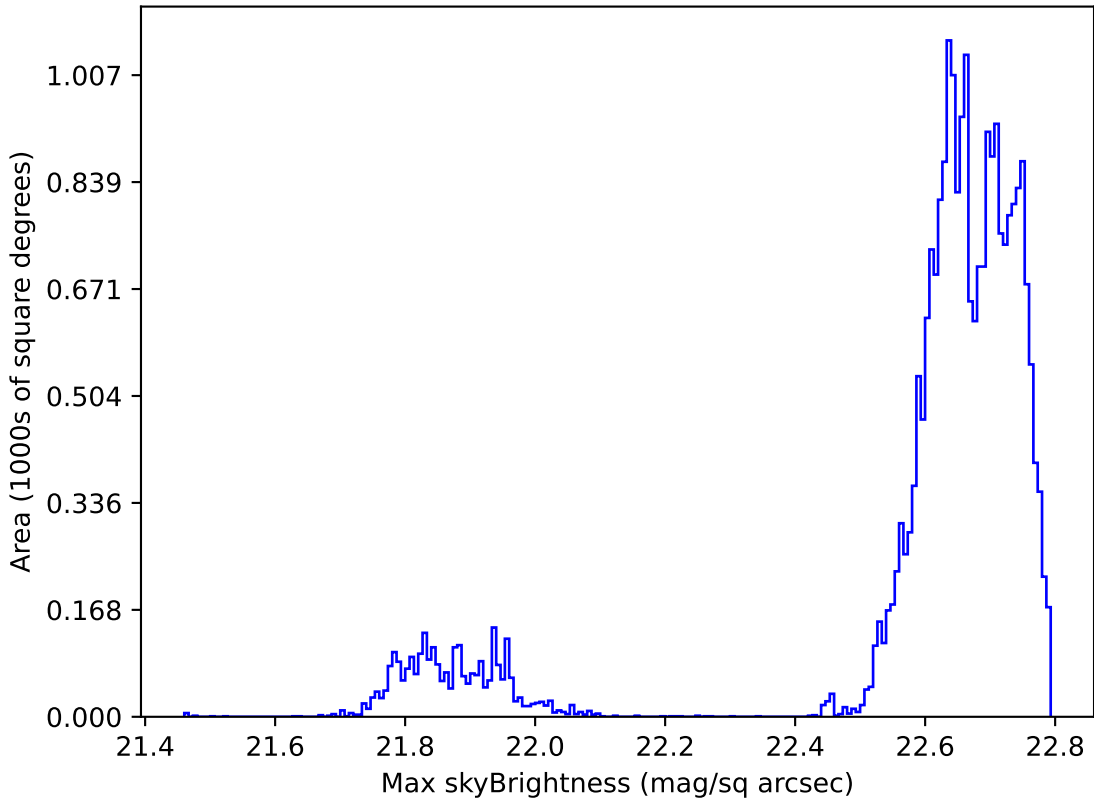
too_elab_heavy_r64_d3_ugrizy_v3.4_10yrs Yr 1 all bands: Max skyBrightness
