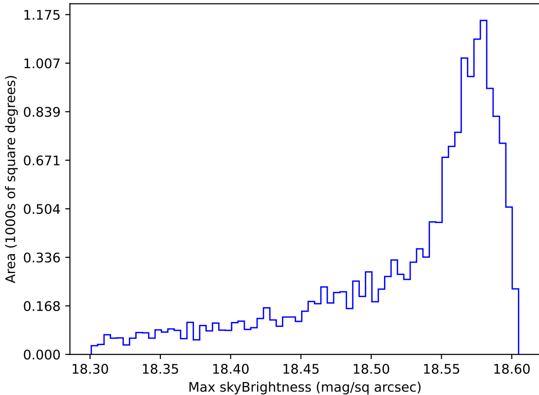
too_elab_heavy_r64_d3_ugrizy_v3.4_10yrs WFD y band: Max skyBrightness
