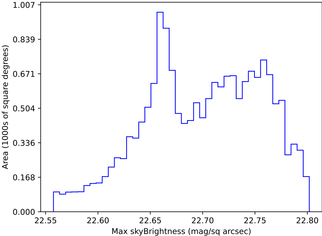
too_elab_heavy_r64_d3_ugrizy_v3.4_10yrs WFD u band: Max skyBrightness
