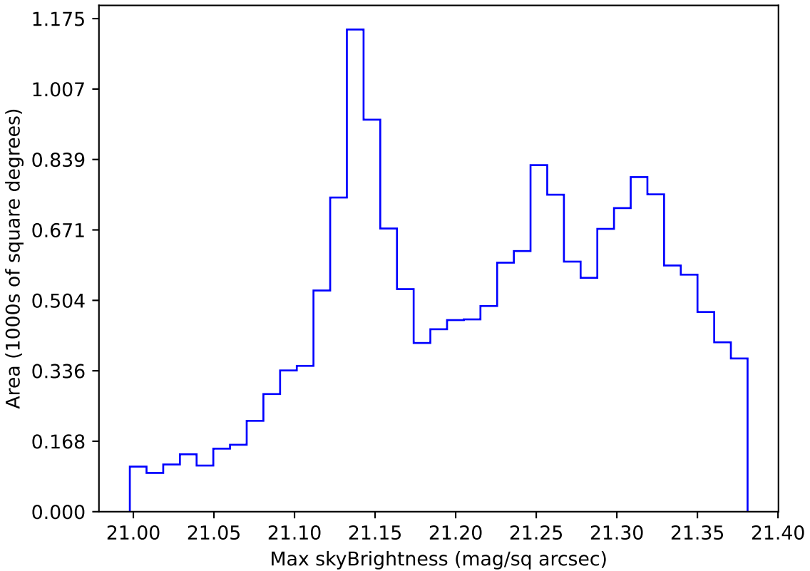
too_elab_heavy_r64_d3_ugrizy_v3.4_10yrs WFD r band: Max skyBrightness
