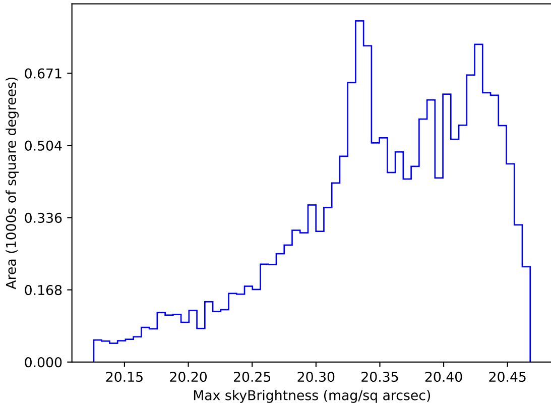
too_elab_heavy_r64_d3_ugrizy_v3.4_10yrs WFD i band: Max skyBrightness
