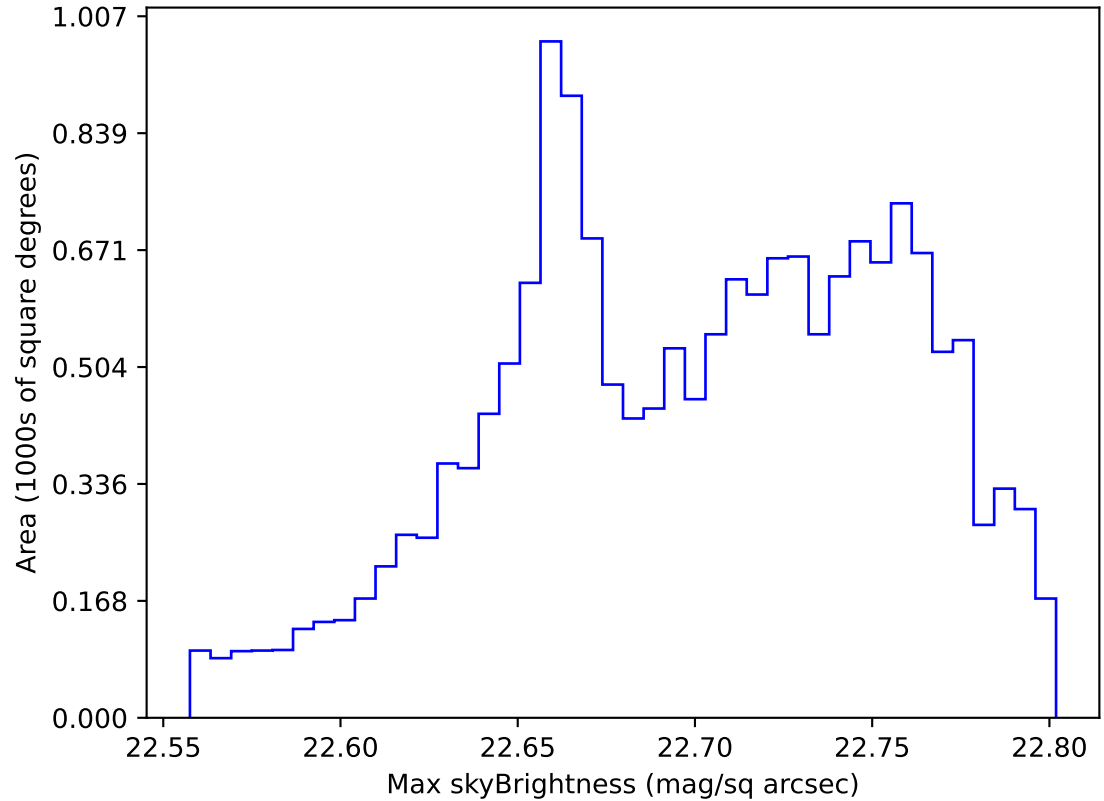
too_elab_heavy_r64_d3_ugrizy_v3.4_10yrs WFD all bands: Max skyBrightness
