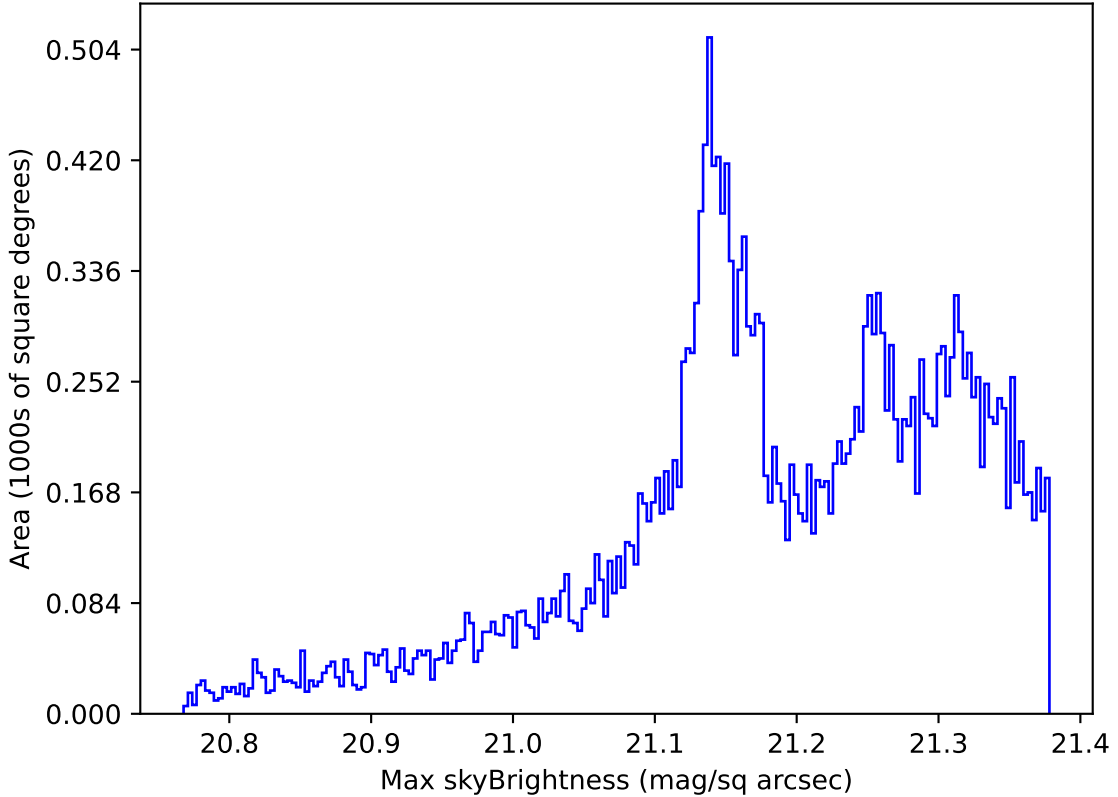
too_elab_heavy_r64_d3_ugrizy_v3.4_10yrs All sky r band: Max skyBrightness
