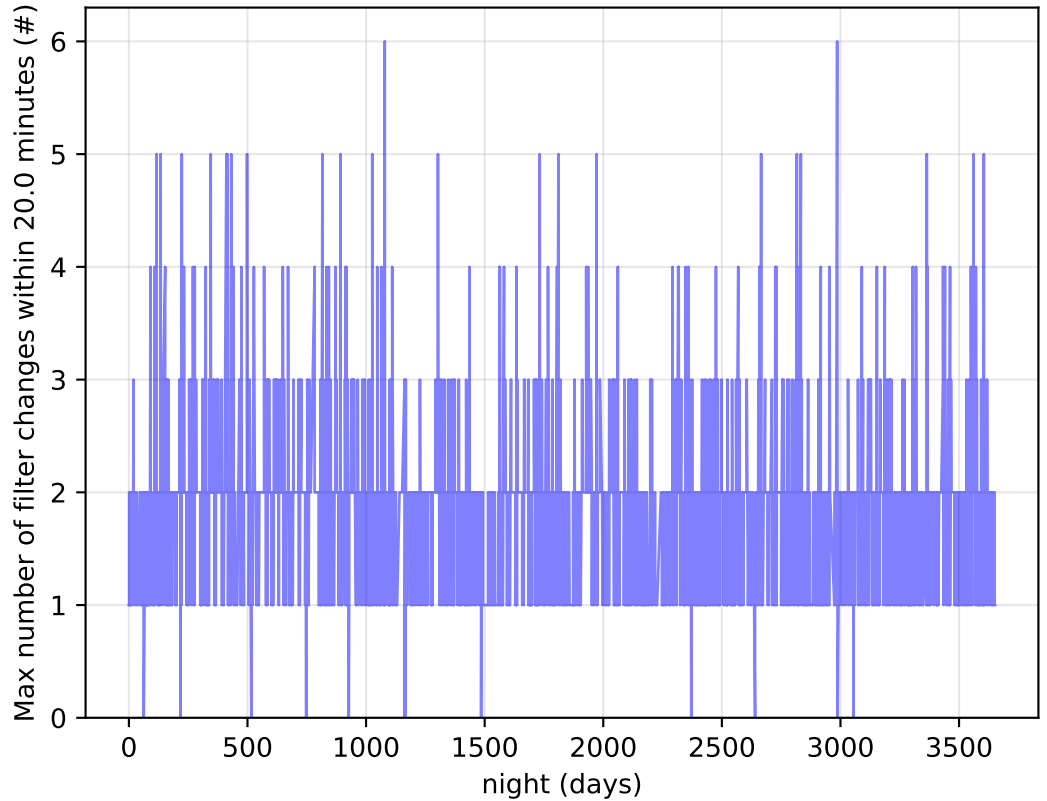
too_elab_heavy_r64_d3_ugrizy_v3.4_10yrs Per Night: Max number of filter changes within 20.0 minutes
