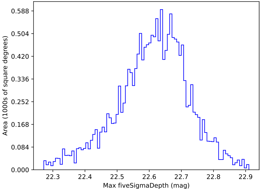
too_elab_heavy_r64_d3_ugrizy_v3.4_10yrs WFD y band: Max fiveSigmaDepth
