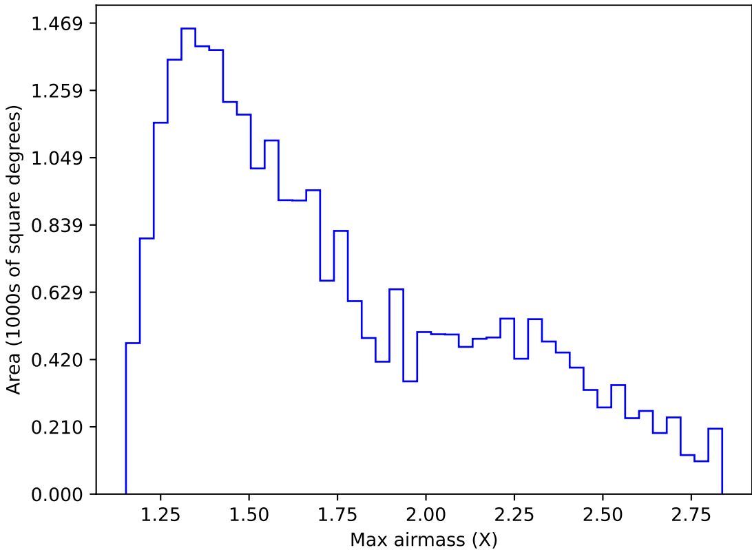
too_elab_heavy_r64_d3_ugrizy_v3.4_10yrs Yr 1 z band: Max airmass
