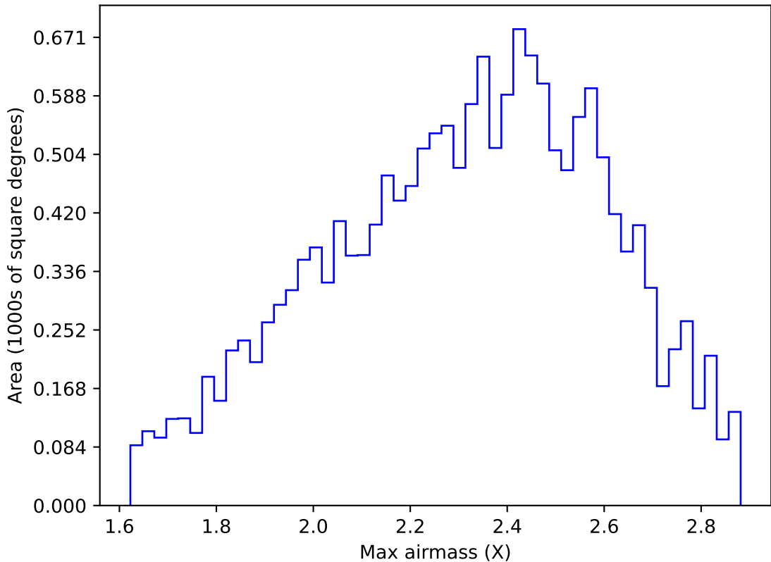
too_elab_heavy_r64_d3_ugrizy_v3.4_10yrs WFD y band: Max airmass
