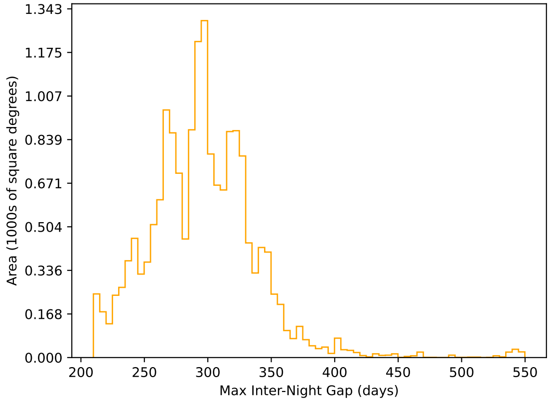
too_elab_heavy_r64_d3_ugrizy_v3.4_10yrs WFD r band: Max Inter-Night Gap
