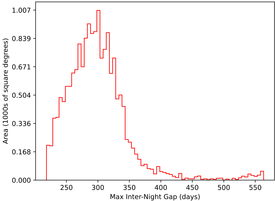
too_elab_heavy_r64_d3_ugrizy_v3.4_10yrs WFD i band: Max Inter-Night Gap
