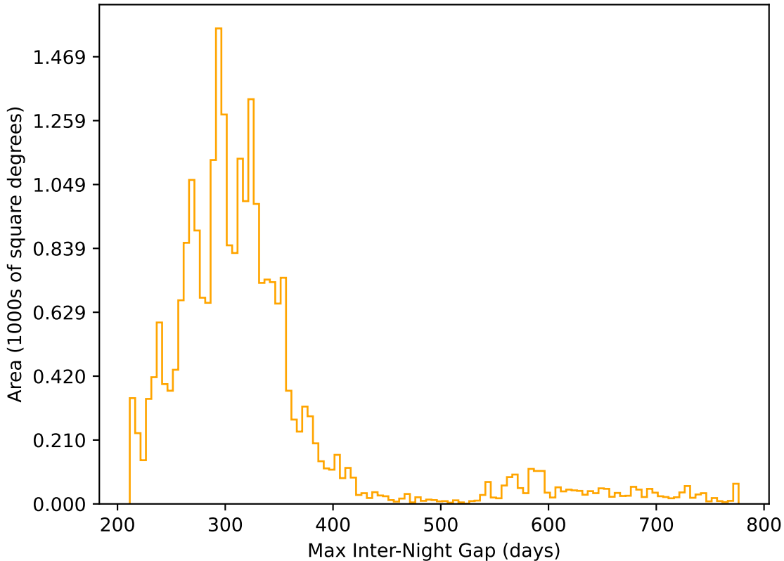
too_elab_heavy_r64_d3_ugrizy_v3.4_10yrs All sky r band: Max Inter-Night Gap
