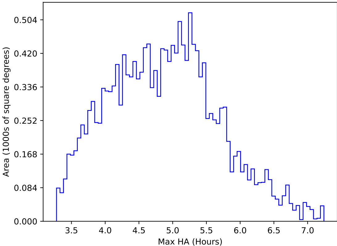
too_elab_heavy_r64_d3_ugrizy_v3.4_10yrs WFD z band: Max HA
